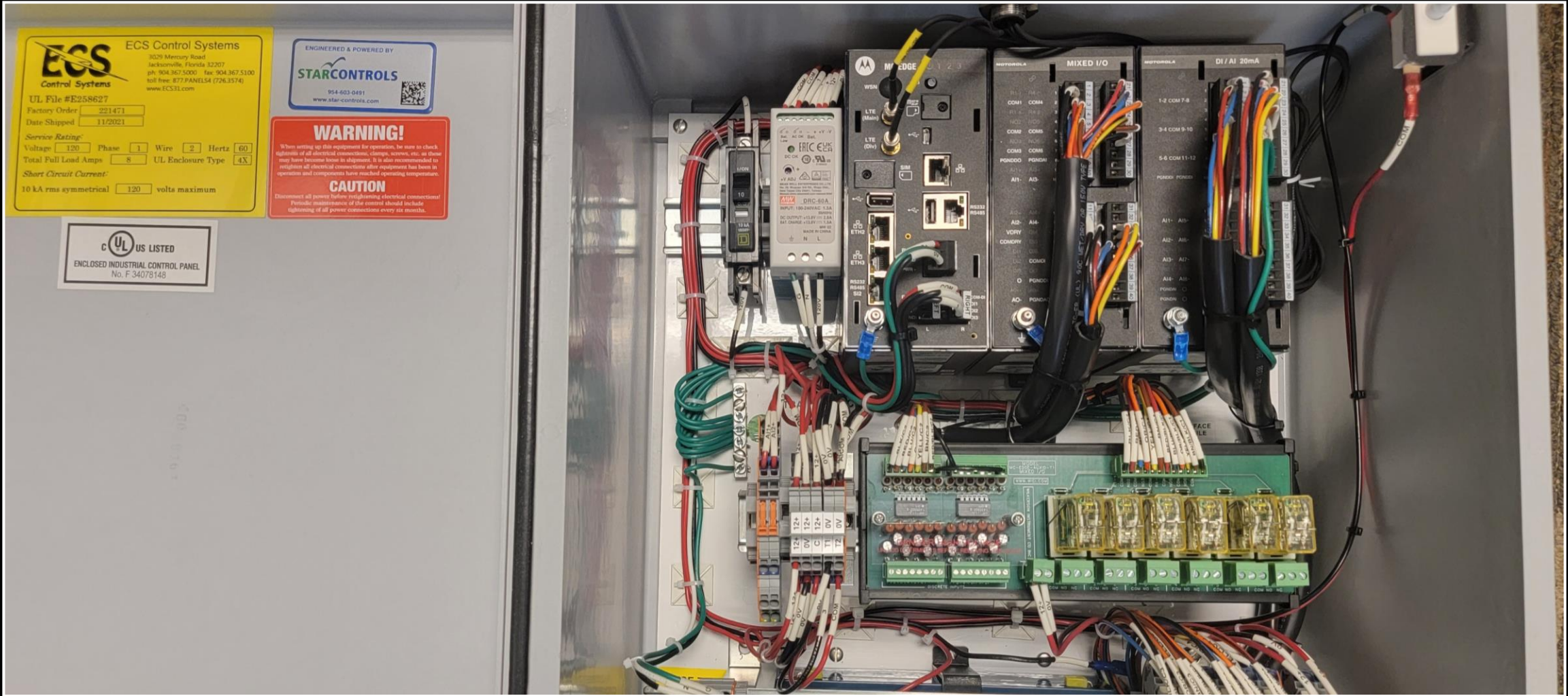
MC-Edge for Monitoring and Control - NEMA-4X Fiberglass
