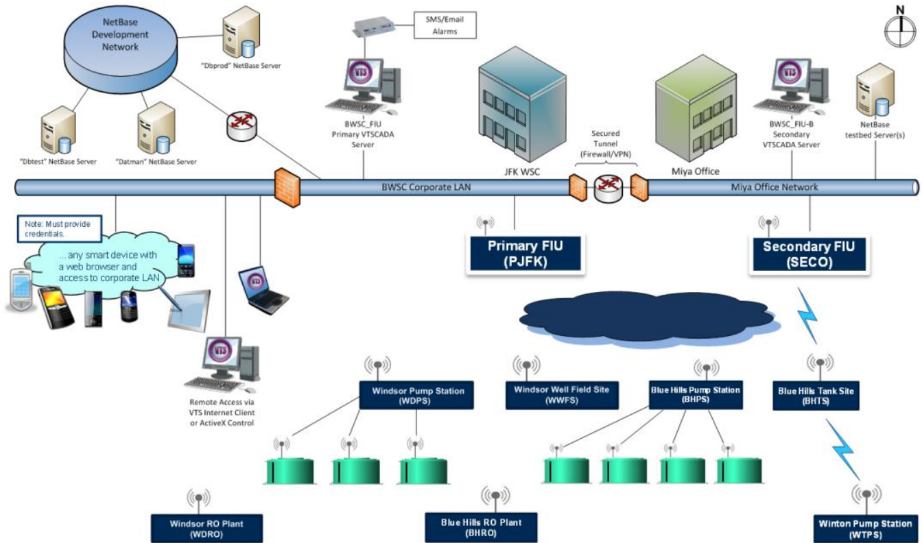
Blue Hills Distribution SCADA System Network Diagram
